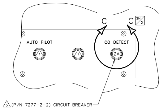
SECTION A SH 2
