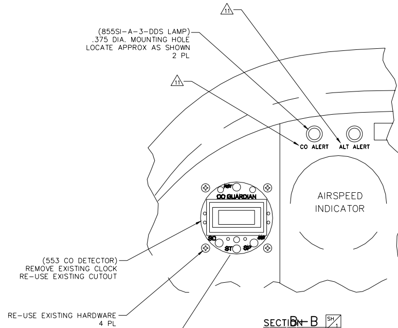
SECTION B SH 2
